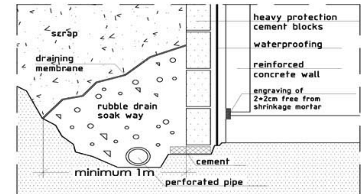
Detail waterproofing earth retaining wall
